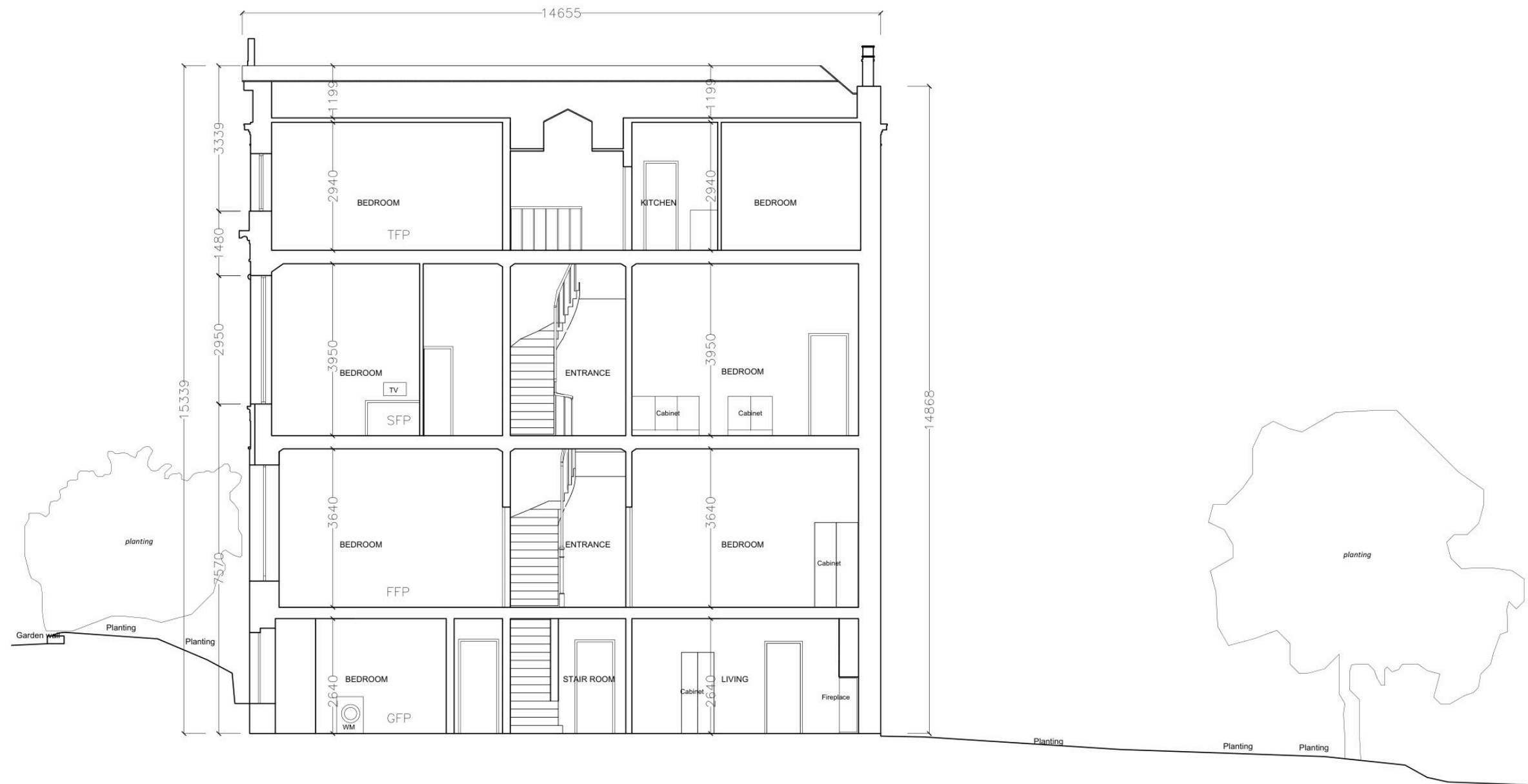
SECTION C-C
